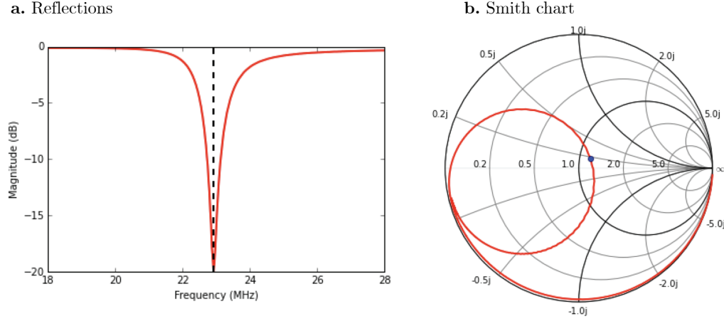
Figure 10: Impedance matching of high power RF antenna. a. Reflected power as a function of frequency. b. Impedance as a function of frequency, visualized on a Smith chart.
