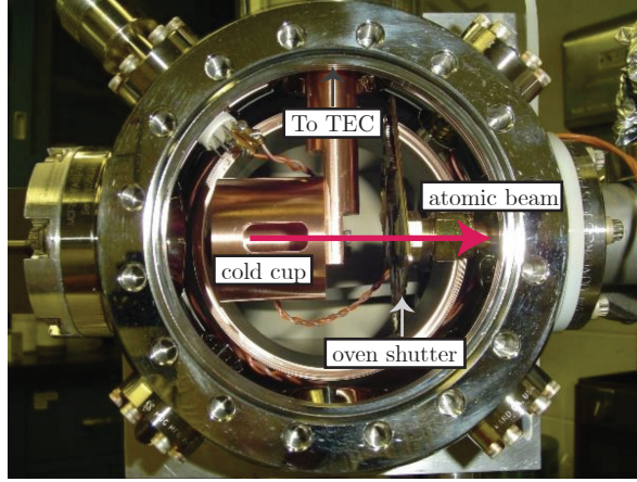
Figure 2: The RbLi oven chamber. We use a cold cup to prevent excess Rb atoms from damaging the ion pumps and a homemade in-vacuum shutter to block the atomic beam after the MOT stage to prevent heating of the atoms at later stages.
