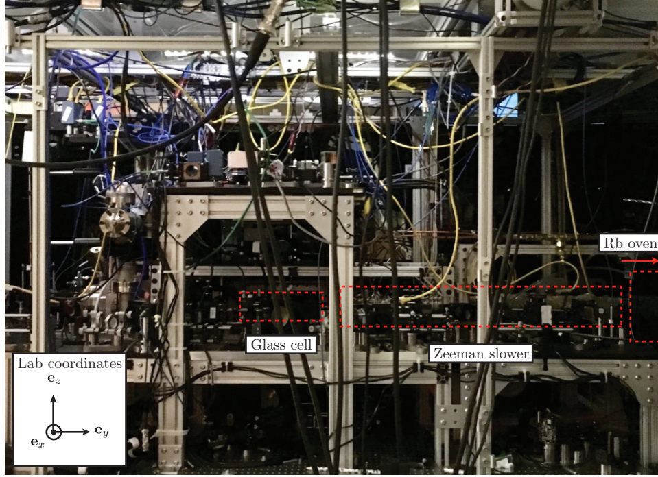
Figure 1: The vacuum system of the RbLi apparatus is divided into an oven, a Zeeman slower and an UHV region containing a glass-cell where all experiments are performed.
