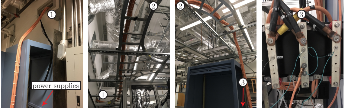
Figure 3: A roller coaster ride, from the power supplies in the service corridor to three copper bars that distribute the power.
