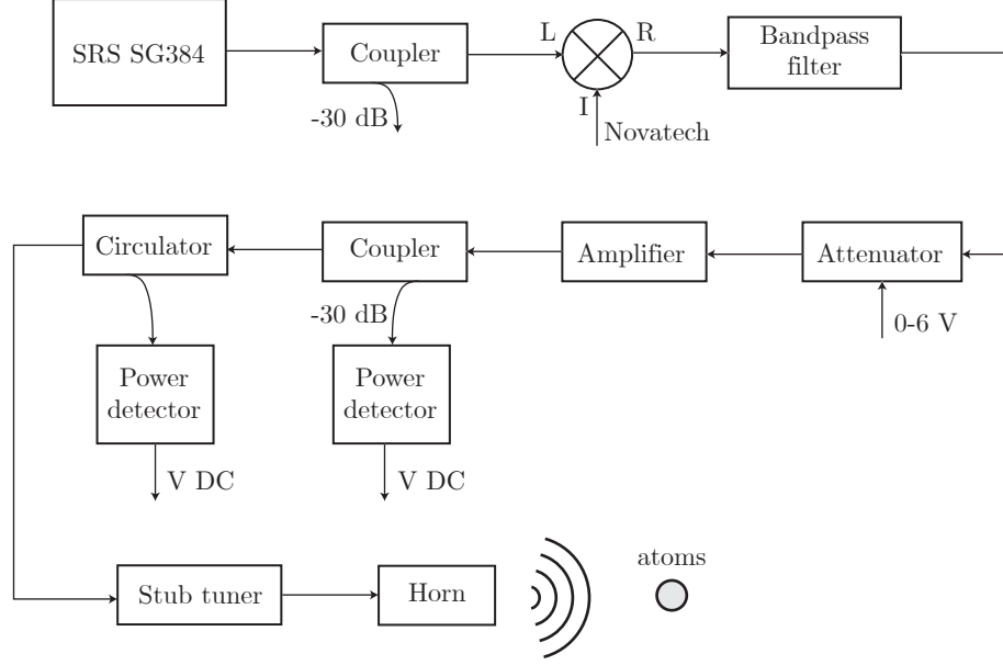
Figure 11: Schematic of 6.8 GHz microwave system.
