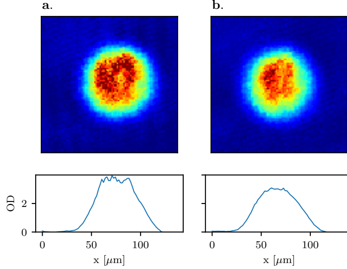
Figure 7: a. A BEC imaged at low intensity shows a ‘flat-top’ density profile. b. In order to recover the Thomas-Fermi profile it is necessary to image high density BECs with intensities larger than I_{\text{sat}} .
