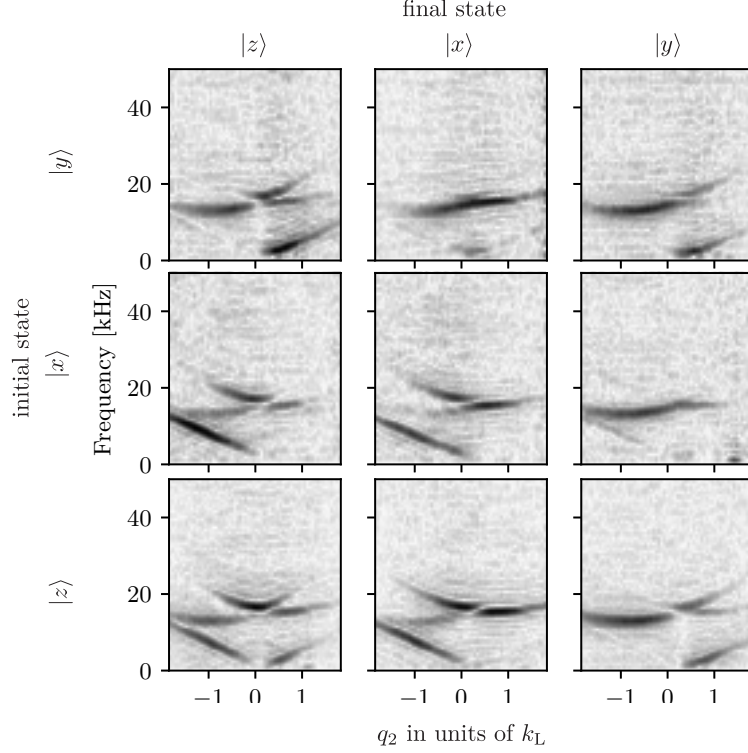
Figure 11: PSD of all the analyzed states as a function of q_2 for fixed q_1 = 0.18 k_L . The different overlaps between the initial state, the Raman dressed states and the measured final state result in peaks with different amplitudes.
