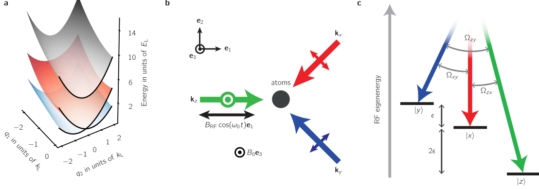
Figure 5: a Our engineered dispersion consisted of a two-level Rashba subspace (red and blue) with a single Dirac point linking the lowest two branches and a topologically trivial higher branch (gray). b We generated |xyz\rangle states by combining a bias magnetic field along \mathbf{e}_3 with an RF magnetic field oscillating along \mathbf{e}_1 . These states were coupled by three cross-polarized Raman laser beams propagating along \mathbf{e}_1 , \mathbf{e}_2 - \mathbf{e}_1 and -\mathbf{e}_1 - \mathbf{e}_2 . c Each pair of Raman lasers was in two-photon resonance with a single transition between the |xyz\rangle states which we coupled strengths (\Omega_{zx}, \Omega_{xy}, \Omega_{yz})/2\pi = (12.6(5), 8.7(8), 10(1)) kHz.
