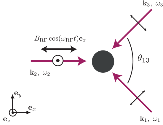
Figure 1: Laser layout: We use a strong RF field and three linearly polarized Raman beams propagating in the xy plane couple the |xyz\rangle states and engineer the Rashba Hamiltonian.
