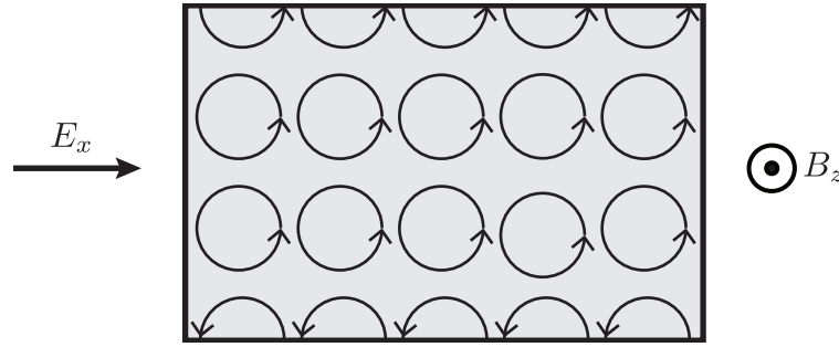
Figure 2: The quantum Hall effect. An electron gas is confined in a two-dimensional material and a strong magnetic field is applied perpendicular to the plane. The electrons on the bulk travel in cyclotron orbits while the electrons on the edge travel 'skipping orbits'.
