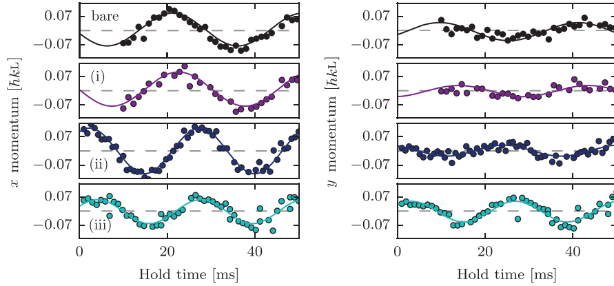
Figure 6: Oscillation of the BEC in the dipole trap along the recoil directions \mathbf{e}_x and \mathbf{e}_y for (top) bare atoms, and the three parameter regimes that we explored (i), (ii), and (iii). We believe that the observed low amplitude oscillations along \mathbf{e}_y are due to the initial detuning ramp not being fully adiabatic.
