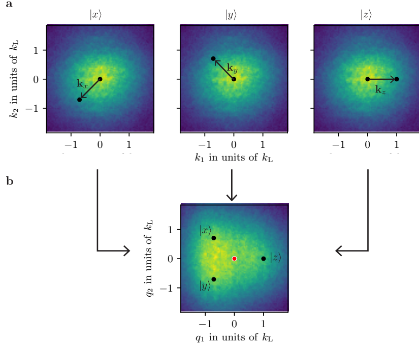
Figure 8: Mapping momentum into quasimomentum: a We used non-condensed atoms with a broad momentum distribution ( T \approx 180 nK and T/T_c \approx 1.1 ). b Atoms in |j, \mathbf{k}\rangle are mapped to Raman dressed states with quasimomentum \mathbf{q} = \mathbf{k} + \mathbf{k}_j . The black dots in the bottom panel represent the location of \mathbf{k} = 0 for each of the |xyz\rangle states and the red dot corresponds to \mathbf{q} = 0 . We performed our experiments starting separately in each of the |xyz\rangle states, which allowed us to sample a larger range of quasimomentum states.
