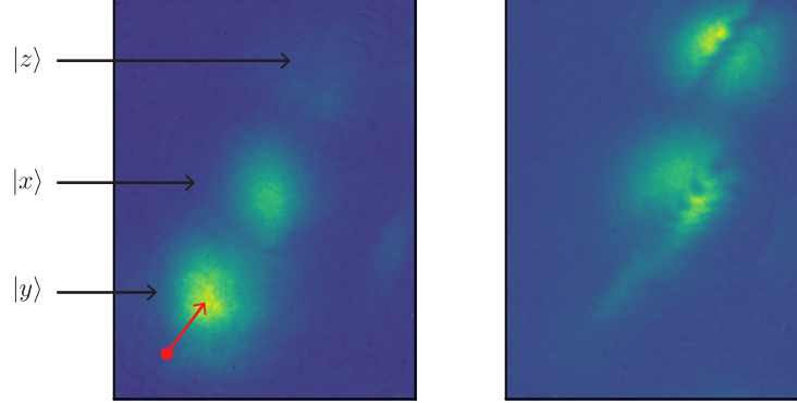
Figure 14: a We prepared atoms in the |y\rangle state such that they are adiabatically mapped to the ground dispersion branch. b We ramped \delta_i and dragged the Dirac point through the atoms.
