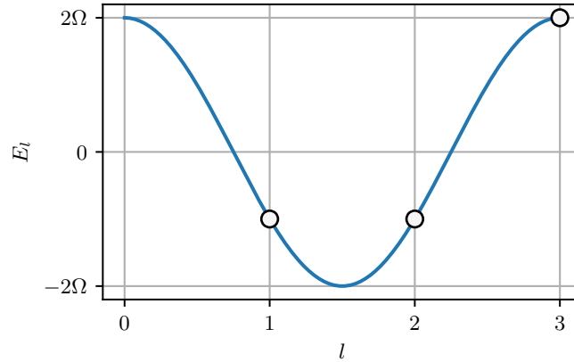
Figure 3: Eigenenergies of Equation 8.5 for q = 0 for N = 3 and \bar{\phi} = 0 . For this particular choice of phase, the energies of the l = 1 and l = 2 states become degenerate
