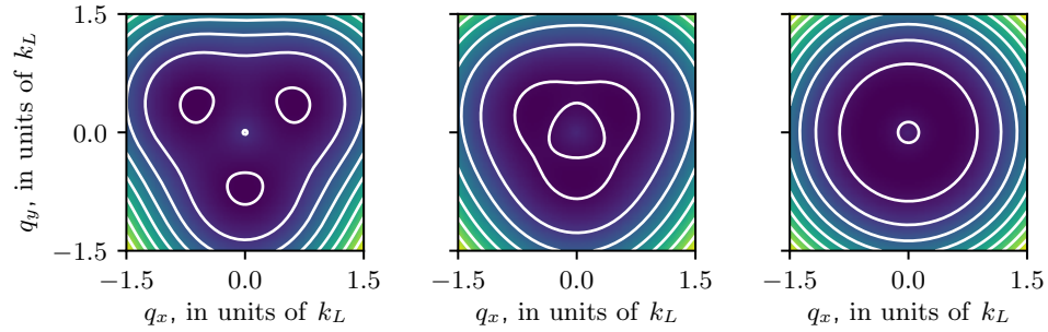
Figure 4: Ground state dispersion relation of Equation 8.5 for N = 3 and \bar{\phi} = 0 for \Omega = 1.75 E_L (left), \Omega = 3.5 E_L (middle) and \Omega = 175 E_L (right). Higher order corrections to \hat{H}^{(0)} decay as 1/\Omega^2 and in the large \Omega limit we recover the Rashba ring dispersion.
