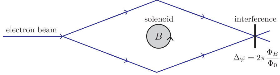
Figure 3: The Aharonov-Bohm experiment. A coherent electron beam is split into two paths surrounding a solenoid which produces a non-zero magnetic field \mathbf{B} inside the gray region and \mathbf{B} = 0 outside. The two beams are later recombined and an interference pattern reveals a phase difference \Delta\varphi = 2\pi\Phi_B/\Phi_0 equal to the magnetic flux enclosed by the electron's path.
