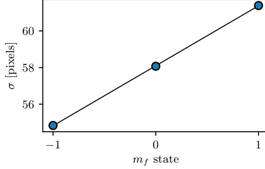
Figure 9: We measured the standard deviation of the momentum distribution along the axis perpendicular to the SG for 10 shots on each m_f state. From the slope of the linear fit we obtain a shearing parameter \alpha \approx \pm 0.067 for m_f = \pm 1 .
