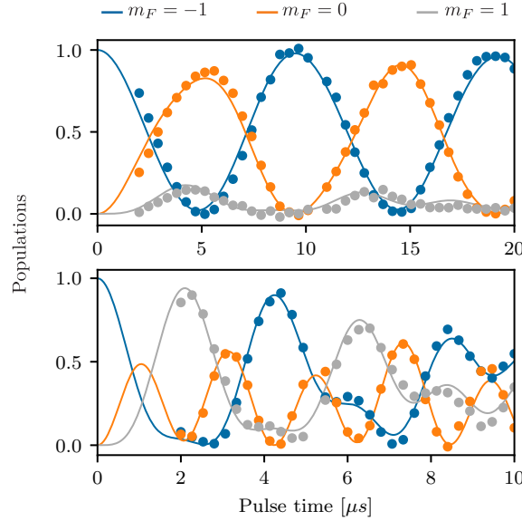
Figure 4: We prepared the system in the |m_F = -1\rangle state and pulsed \Omega for variable times. We used a least squares minimizer to fit the populations in the |m_F\rangle states as a function of pulsing time to get an initial estimate of \Omega . The top panel shows the time evolution of \Omega/2\pi \approx 76 kHz and the bottom panel shows the evolution for \Omega/2\pi \approx 238 kHz
