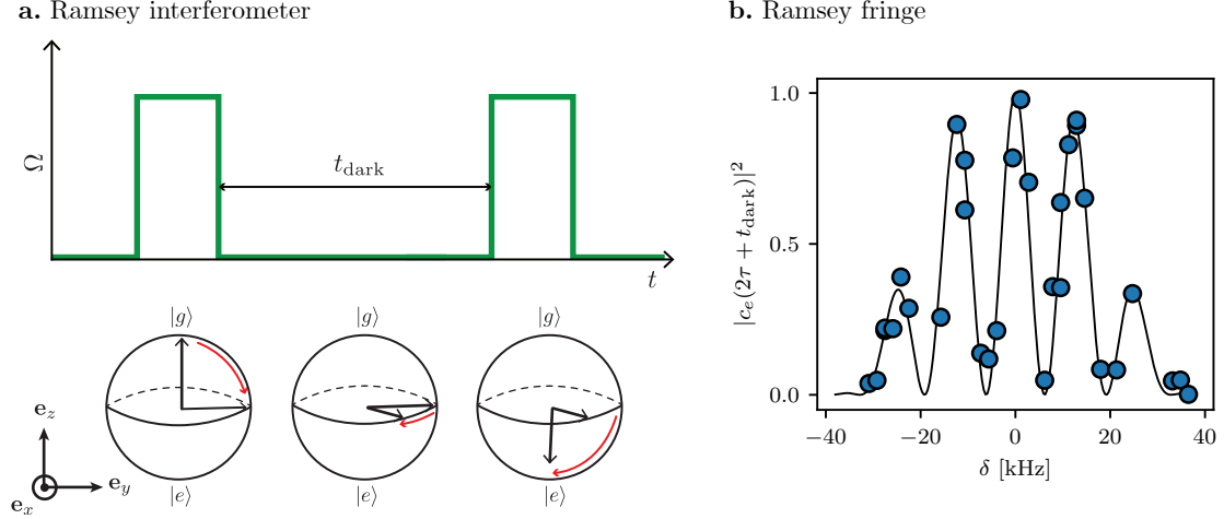
Figure 11: a. A Ramsey interferometer: Two \pi/2 pulses are separated by a time t_{\text{dark}} . The phase accumulated in the interferometer is equal to the detuning multiplied by the dark time. b. A Ramsey interference fringe. Data (blue dots) and fit (black line) obtained from coupling two levels using an RF field with \Omega = 1 kHz. We applied a pair of \tau = 25 \mu\text{s} pulses separated by a 50 \mu\text{s} wait and varied the detuning by changing the bias magnetic field.
