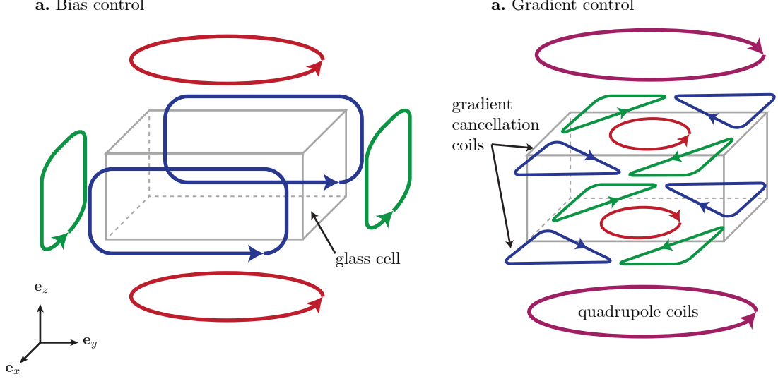
Figure 4: Magnetic coil geometry in the RbLi apparatus a. We use three pairs of Helmholtz coils to produce bias fields along \mathbf{e}_x , \mathbf{e}_y and \mathbf{e}_z . b. We have a pair of coils that produce strong quadrupole magnetic fields for the MOT and magnetic trapping. Additionally we have a pair of ‘cloverleaf’ coils to control the gradients in B_z .
