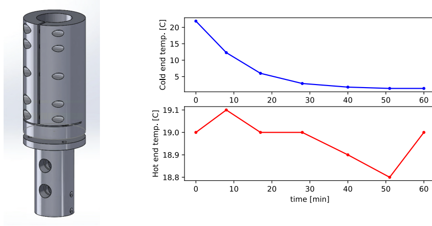
c. Testing prototype oven and heat sink
