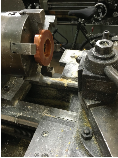
a. Coil mounted on lathe
