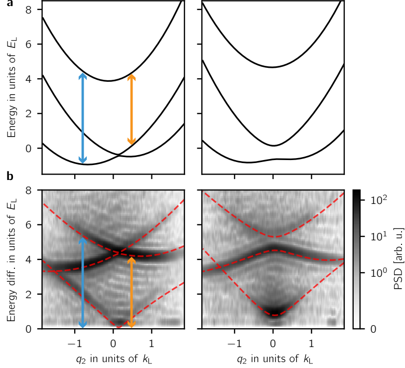
Figure 12: a Predicted dispersion relation as a function of q_2 for fixed q_1 = -0.09 k_L (left) and 0.65 k_L (right), computed for the experiment parameters. The energy differences between the branches enclosing the vertical arrows appear as peaks in the spectral maps below. b Power spectral density (PSD) for the same parameters as above which we obtained by Fourier transforming the populations in the |xyz\rangle states with respect to t_p . The dashed lines correspond to the energy differences computed using the dispersion curves on the top panel.
