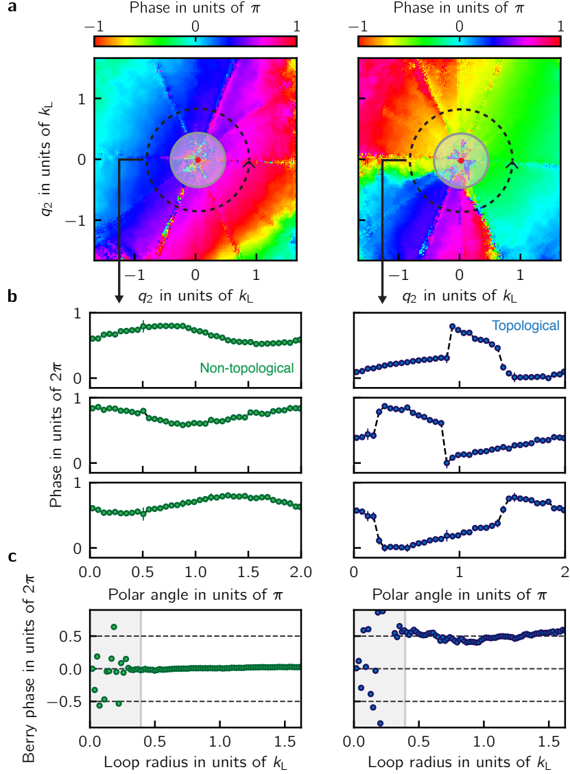
Figure 17: Topological invariants from quantum state tomography, for the non-topological branch ( n = 3 , left) and the topological branch ( n = 1 , right). a Phase differences as a function of quasimomentum from the z \rightarrow x transition b Phase differences as a function of polar angle for a loop radius 0.77 k_L from the z \rightarrow x (top), x \rightarrow y (middle) and y \rightarrow z (bottom) transitions. The phases associated with the topological branch are characterized by two \pi valued discontinuities. Each row of phases was shifted by a constant value so that the three rows of phases share the same vertical axis. All phases shown here were binned and averaged using the fit uncertainties as weights. c Inferred Chern number as a function of loop radius. For loops with q > 0.4 k_L we obtained an integrated Berry phase and asymptotic Chern number of \Phi_B/2\pi = 0.01(1) for the non-topological branch and \Phi_B/2\pi = 0.5(5) for the topological branch.
