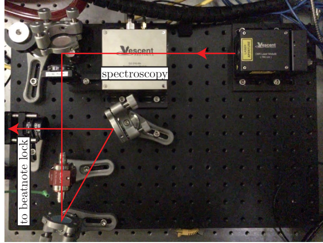
Figure 5: Master laser system. We replaced the old Vortex II laser with a Vescent photonics DBR Laser Module System that is considerably more stable.
