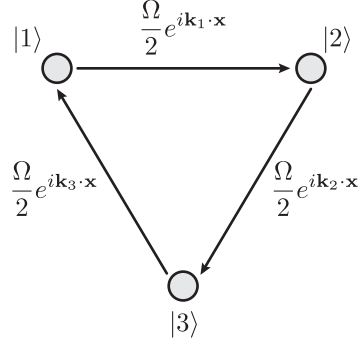
Figure 2: The Rashba ring coupling. To generate Rashba SOC in a system of cold atoms it is necessary to cyclically couple N \geq 3 internal states such that the transition |j\rangle \rightarrow |j+1\rangle has a momentum transfer \mathbf{k}_j and \sum_j \mathbf{k}_j = 0 such that there is no momentum transfer for a closed loop |1\rangle \rightarrow |2\rangle \dots |N\rangle \rightarrow |1\rangle . The ring coupling combined with the free particle Hamiltonian give rise to a 2-level subspace that can be described to first order by the Rashba Hamiltonian
