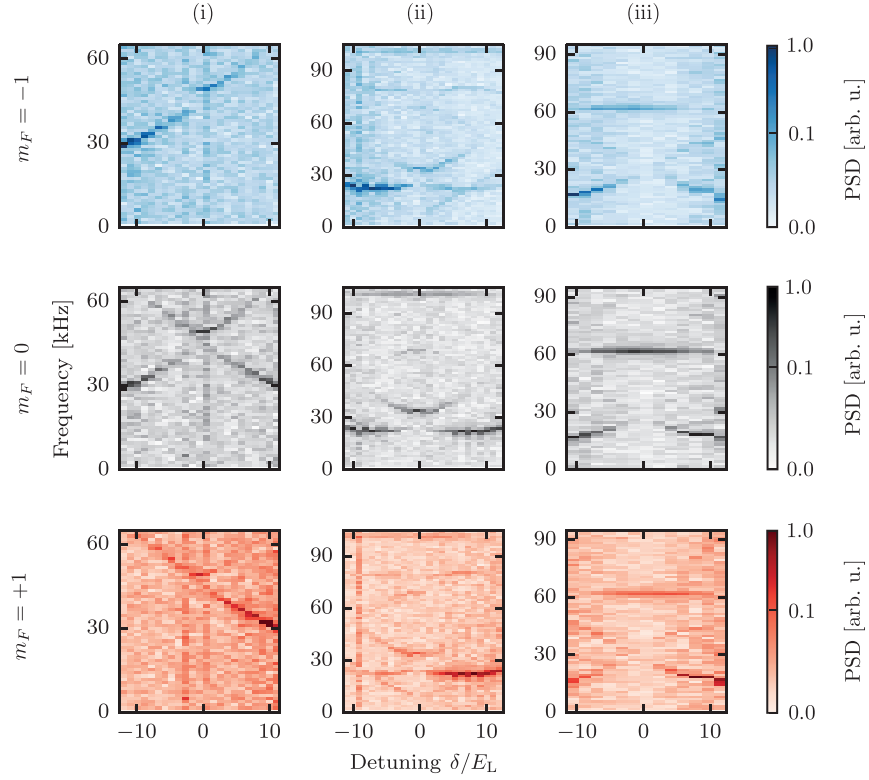
Figure 5: Power spectral density of the time dependent occupation probability for each state in the measurement basis for three coupling regimes: (Left) \Omega_0 = 9.9E_L , \Omega = 0 , (Center) \Omega_0 = 0 , \Omega = 8.6E_L , \delta\omega = \epsilon + 12E_L , and (Right) \Omega_0 = 4.9E_L , \Omega = 8.4E_L , \delta\omega = \epsilon + 17E_L . Each panel is normalized to peak amplitude to highlight small amplitude features in the PSD of the periodically driven SOC, and the highest value on the frequency axis corresponds to the FFT bandwidth.
