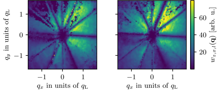
Figure 16: Two sample weight arrays w_{i,j,l}(\mathbf{q}) for i, j = z, x and atoms prepared in the topological dispersion branch. We obtained the weights using the uncertainties from the fits and the trajectory of the Dirac point during the state preparation. We combined the weights and the phase differences \Delta\phi_{n,i,j,l} obtained from the time dependent fits using Equation 8.18 to obtain the phase maps displayed in Figure 17a
