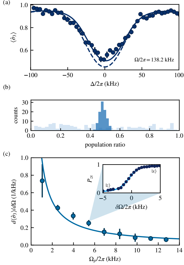
Figure 11: (a) The fractional population imbalance of the \downarrow\uparrow transition for \Omega/2\pi = 138.2(1) kHz over detuning \Delta . The dashed curve is calculated using Equation 6.7 and the solid one using the full Breit-Rabi expression. (b) The fidelity of preparing a balanced superposition of |\downarrow\rangle and |\uparrow\rangle (dark blue) states compared to |m_F = 0\rangle and |m_F = -1\rangle states (light blue). (c) The robustness of \downarrow, \uparrow transition against fluctuations \delta\Omega for different probe field coupling strengths. The points represent the slope of the fitted curves to the fractional population imbalance (inset).
