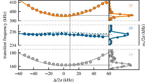
Figure 5: Spectroscopic data showing transitions between the |xyz\rangle states for \Omega/2\pi = 194.5(1) kHz. The vertical scale of the center panel ( zx transition) has only 10% the range of the other panels. The dashed lines correspond to the Hamiltonian of Equation 6.1 while the solid lines include the dependence of the quadratic shift on \Delta . Right: representative spectra.
