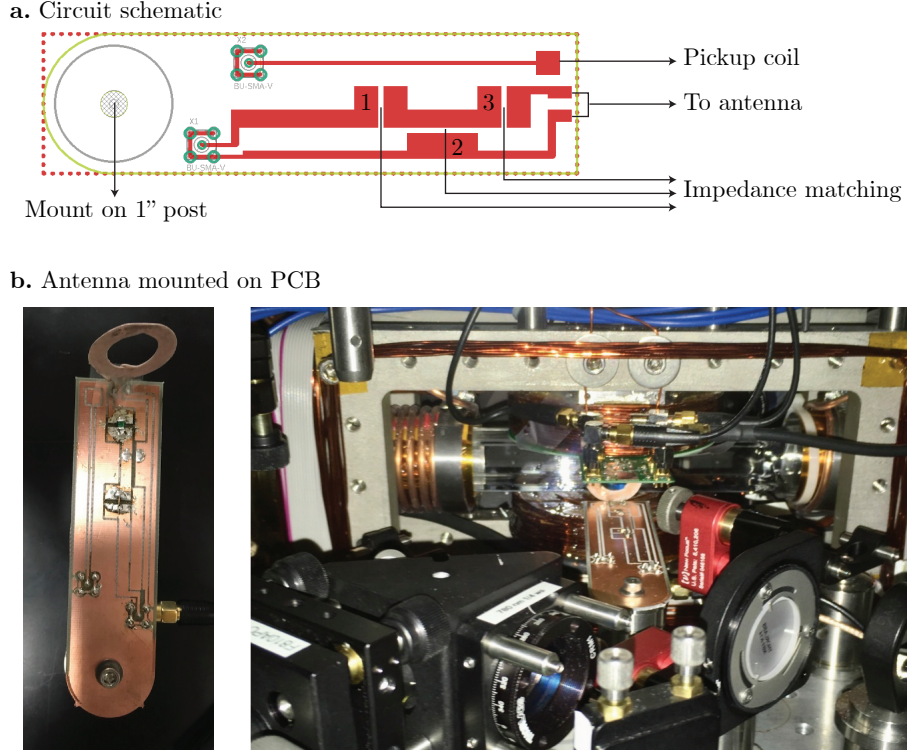
Figure 9: We use a commercial resonator with an impedance matching network to produce high power RF fields. a. Diagram of the impedance matching network. b. A picture of the resonator mounted on a PCB. We place this device as close to the atoms as possible next to the glass cell.
