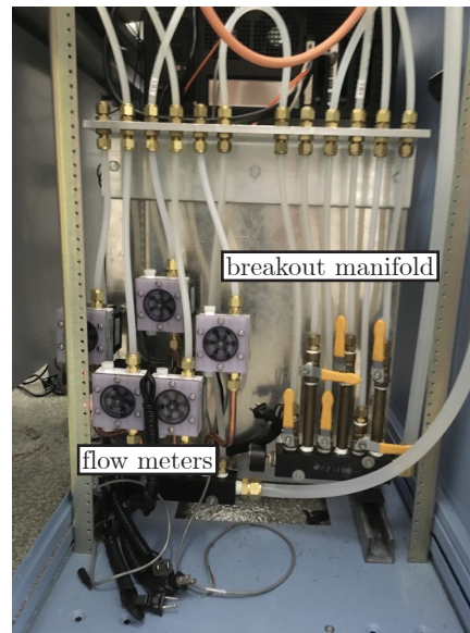
Figure 1: Water cooling
