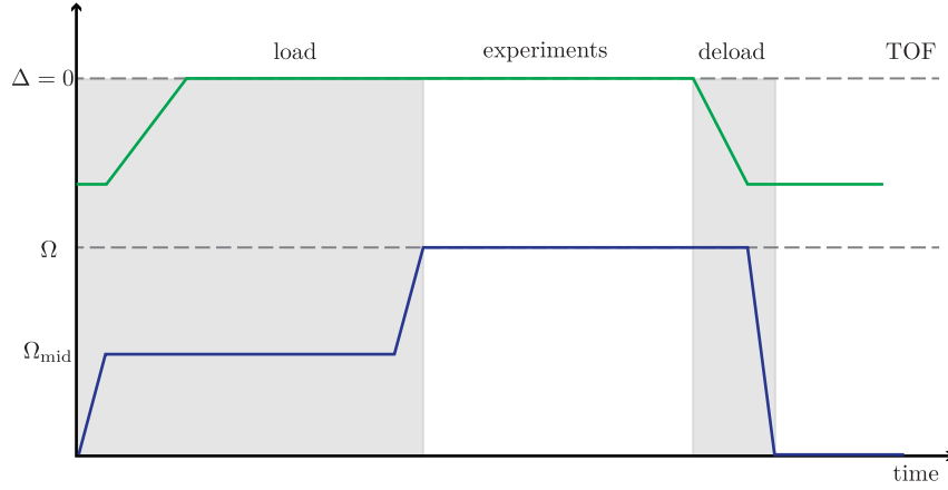
Figure 3: Detuning and RF coupling strengths ramps (not to scale) performed to adiabatically prepare the |xyz\rangle states starting in the |m_F\rangle states and vice versa.
