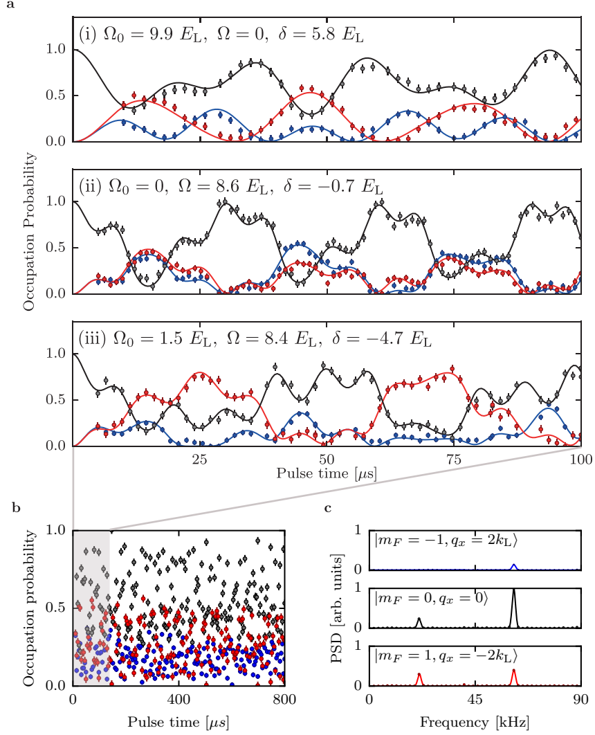
Figure 4: a. Occupation probability for the three states in the measurement basis |m_F = -1, q = q_x + 2k_L\rangle (blue), |m_F = 0, q = q_x\rangle (black), and |m_F = +1, q = q_x - 2k_L\rangle (red), following unitary evolution under \hat{H}_{\text{SOC}} for times up to 100 \mu\text{s} at different spin-orbit coupling regimes: (i) \Omega_0 = 9.9 E_L, \Omega = 0, \delta = 5.8 E_L , (ii) \Omega_0 = 0, \Omega = 8.6 E_L, \delta = -0.7 E_L, \delta\omega = \epsilon + 12 E_L , and (iii) \Omega_0 = 1.5 E_L, \Omega = 8.4 E_L, \delta = -4.7 E_L, \delta\omega = \epsilon + 17 E_L . b. Occupation probability for long pulsing up to 800 \mu\text{s} for parameters as in (iii). c. Power spectral density of the occupation probability. We subtract the mean value of each probability before taking the Fourier transform to remove peaks at f = 0 . The peaks in the PSD then correspond to the relative eigenenergies of \hat{H}_{\text{SOC}} .
