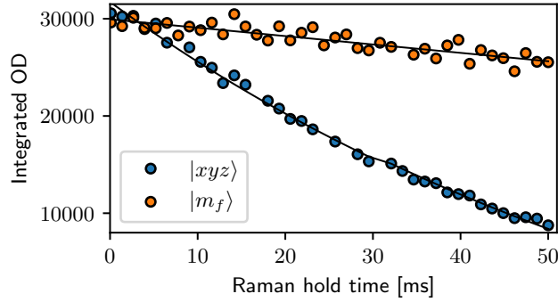
Figure 7: Lifetime of Raman dressed states. We Raman dressed atoms in the |m_f\rangle and |xyz\rangle states. The orange markers correspond to atoms initially prepared in |m_f = -1\rangle (no high power RF involved) and the blue markers correspond to atoms |xyz\rangle (three averaged traces). The lifetime of doubly dressed states is significantly reduced as compared to the lifetime of the Raman dressed |m_f\rangle states, indicating that of resonant scattering of photons is not our only loss mechanism.
