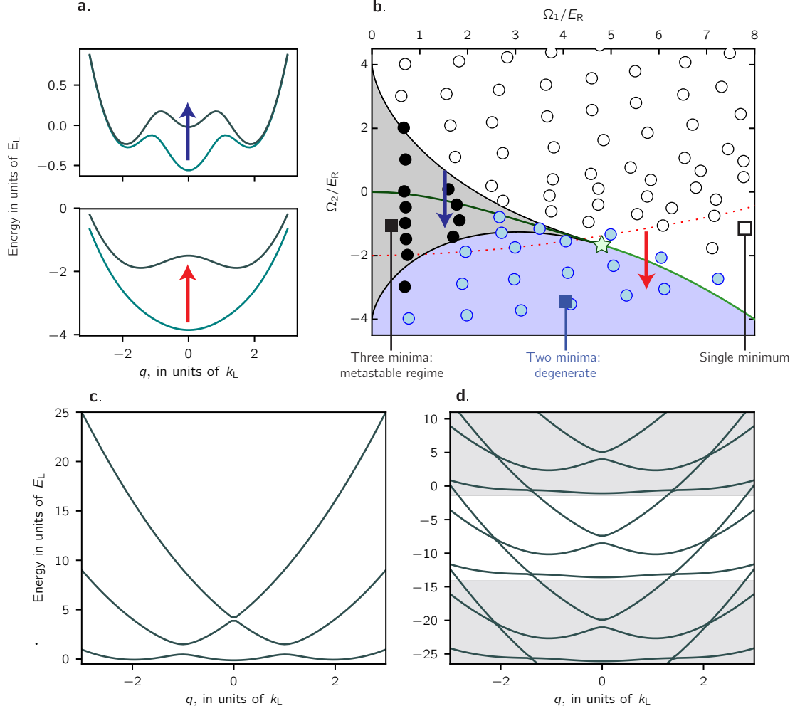
Figure 12: Magnetic phases of a spin-1 SOC system. a. Ground state energies of a spin-1 SOC system for \Omega_1 = 1.5 E_L (top) and \Omega_2 = 1.5 E_L (bottom). By changing \Omega_2 we moved the location of the central minima. b. Phase diagram of a spin-1 SOC system. The green line corresponds to a line of phase transitions where the system goes from magnetized to unmagnetized. c. Dispersion relation of effective Hamiltonian computed for \Omega_1 = 2 E_L , \Omega_2 = 0 . d. Floquet quasienergy dispersion relation for the same parameters. The magnitude of \Omega_1 effectively modifies \Omega_2 in the RWA Hamiltonian.
