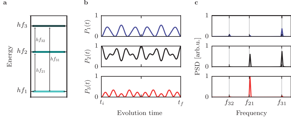
Figure 1: a. Eigenenergies of a three-level system described by \hat{H}'(\Omega_1, \Omega_2, \Omega_3) . b. The system is prepared in |\psi_2\rangle and subjected to \hat{H}' at time t_i . The three panels show the occupation probabilities of the states |\psi_1\rangle (blue), |\psi_2\rangle (black), and |\psi_3\rangle (red) in the measurement basis, for evolution times up to t_f . c. Power spectral density of the occupation probabilities from panel b. The three peaks in the Fourier spectra correspond to the energy differences present in panel a.
