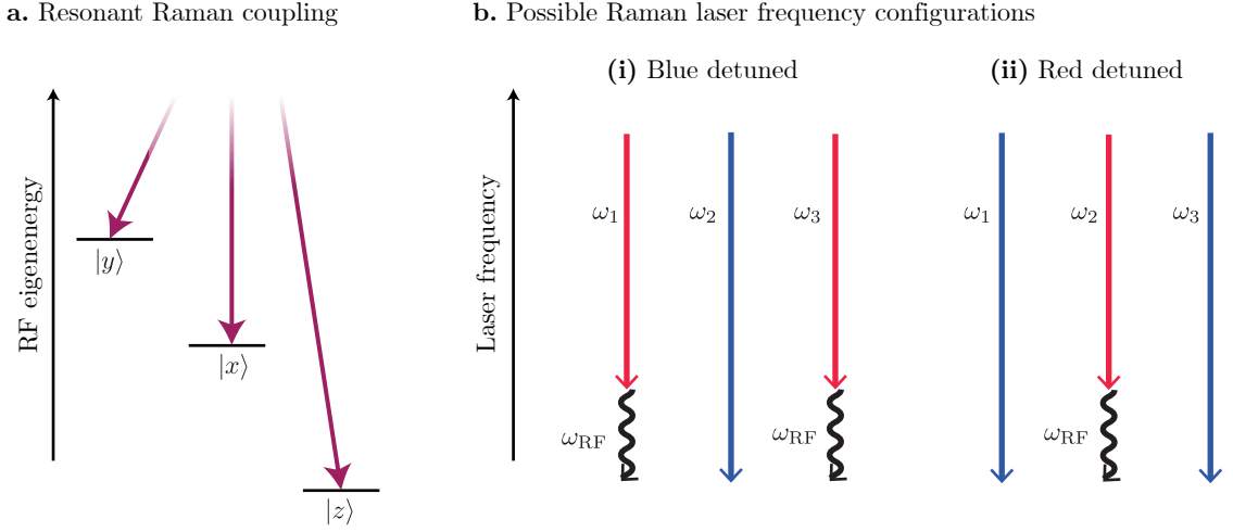
Figure 2: a The choice of laser frequencies should be such that in the frame rotating with frequency \omega_{\text{RF}} we get resonant Raman coupling of the |xyz\rangle states. b. Possible laser frequency configurations: i) Blue detuned configuration: There are 2 frequencies smaller by about \omega_{\text{RF}} and one larger frequency. ii) The red detuned configuration: there are 2 frequencies that are larger by about \omega_{\text{RF}} and one smaller frequency.
