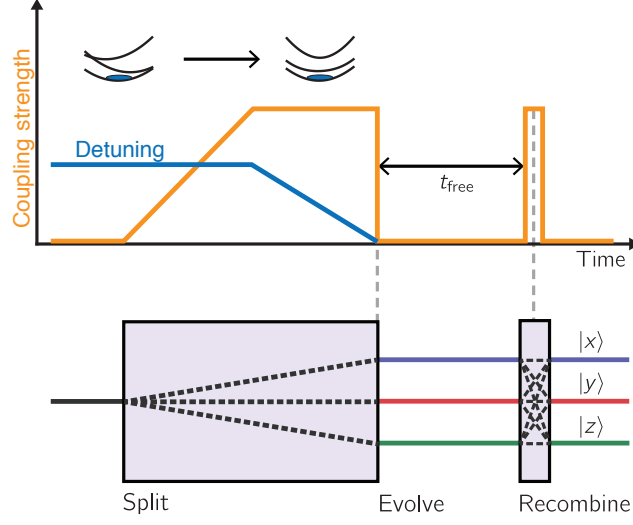
Figure 13: Experimental protocol for three-arm Ramsey interferometer (not to scale). (Top) We started with atoms in state |z, y, \mathbf{q}_i = \mathbf{k} + \mathbf{k}_j\rangle and with detuning \delta_y = \pm 5 E_L and \delta_z = \pm 5 E_L . We ramped the Raman lasers on in 750 \mu s and then ramped the detuning to nominally zero. We let the system evolve in the dark for times between 5 \mu s and 400 \mu s , followed by a 25 \mu s Raman pulse. (Bottom) The implemented experimental protocol was equivalent to a three-arm interferometer that split an initial state into three final states with amplitudes related to the initial wave function phases.
