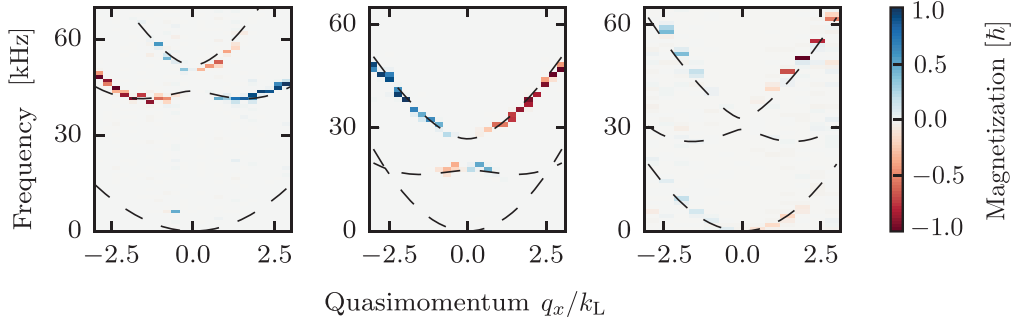
Figure 8: Spin-dependent SOC dispersion for three different coupling regimes. We combine the PSD of the occupation probability of the states |m_F = \pm 1, q_x = \mp 2k_L\rangle , and shift each frequency by an amount proportional to the squared quasimomentum and the effective mass. The dashed lines are the calculated Floquet energies for the Hamiltonian using our calibration parameters.
