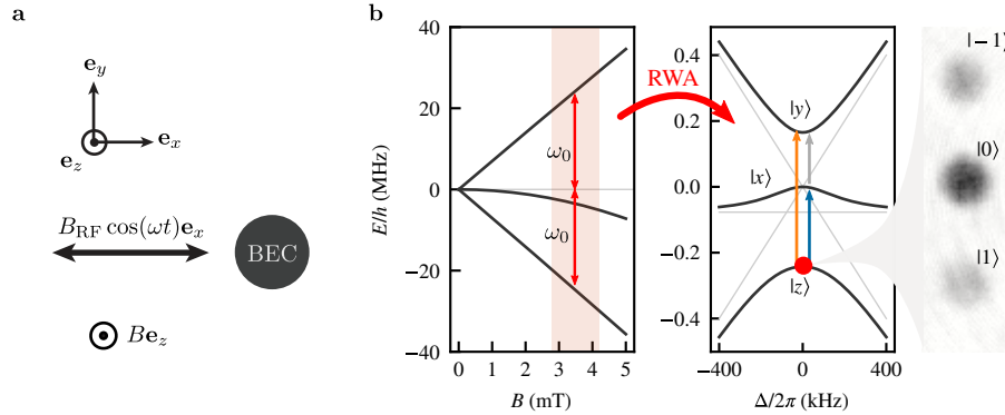
Figure 1: a. Setup for implementing CDD using a strong RF magnetic field. b. Left: dependence of the 5^2S_{1/2} , F = 1 ground state of ^{87}\text{Rb} on magnetic field, where the quadratic dependence of the |m_F = 0\rangle state’s Zeeman shift has been exaggerated so it is visible on the same scale. Center: energies of the |xyz\rangle eigenstates, for \Omega/2\pi = 200 kHz (black curves) and \Omega = 0 (grey curves). Right: TOF absorption image of |z\rangle at \Delta = 0 , showing the constituent |m_F\rangle states.
