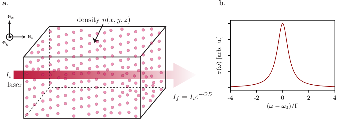
Figure 5: a. A laser beam traveling along \mathbf{e}_z through a medium with density n(x, y, z) . The intensity decays exponentially with the integrated column density and the scattering cross section \sigma\omega . b. The scattering cross section has a Lorentzian line shape with a full width half maximum equal to \Gamma .
