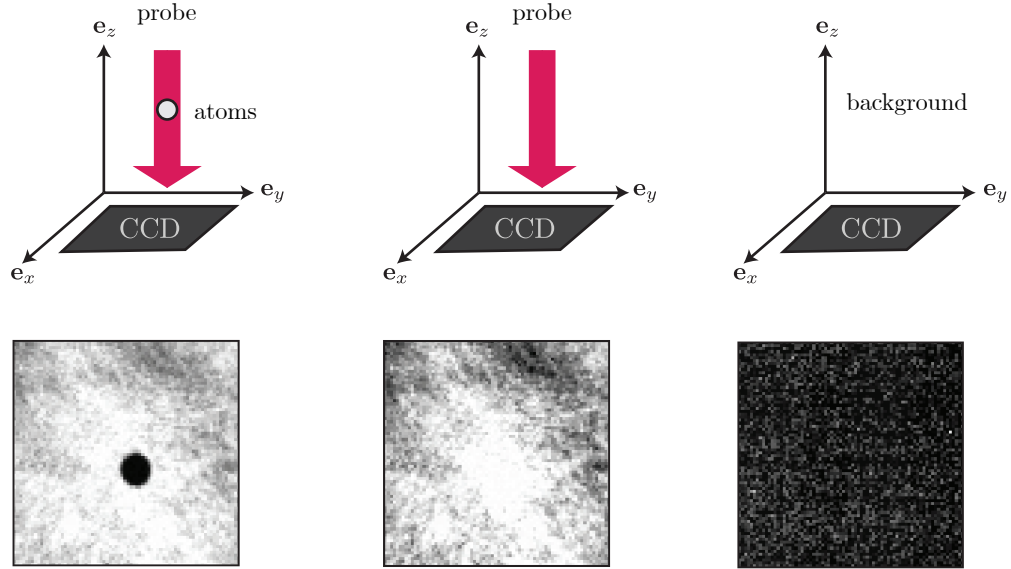
Figure 6: Resonant absorption imaging. An atomic sample is illuminated with a resonant probe whose intensity is later recorded on a CCD camera. Two additional images of the unabsorbed probe intensity and the background intensity are captured in order to reconstruct the optical density of the atoms.
