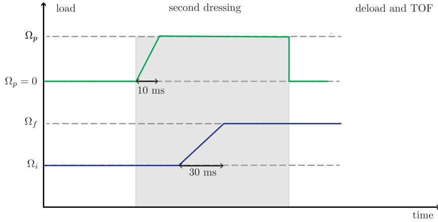
Figure 10: Experimental protocol for implementing concatenated CDD. We started an initial RF coupling strength \Omega_i and ramped on the probe field \Omega_p in a few ms with \omega_p = \omega_{z,x}(\Omega_f) so that it was initially slightly off resonant with the zx transition. We then ramped the RF field to \Omega_f , brining \omega_p to resonance.
