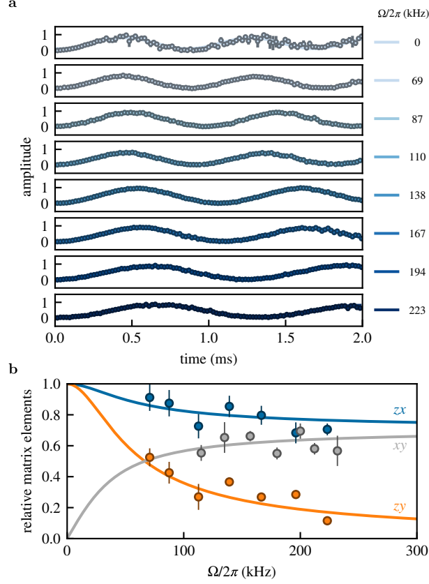
Figure 8: a. Rabi oscillations. Phase coherence is maintained throughout the oscillations in the dressed basis, while it is quickly lost in the |m_F\rangle basis. The marker size reflects the typical uncertainties on the dressed basis oscillations. b. Relative transition matrix elements measured by driving Rabi oscillations between all the |xyz\rangle states at constant probe power for different values of \Omega . The zx (blue) and zy (orange) transitions decrease monotonically with increasing \Omega for \Delta = 0 , while they increase for xy .
