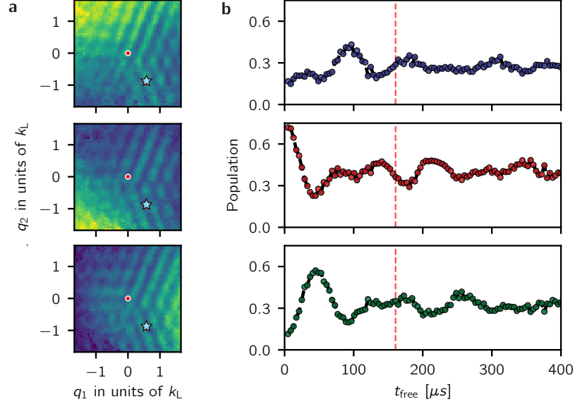
Figure 15: a Probabilities as a function of quasimomentum for the three output ports of the interferometer at t_{\text{free}} = 160 \mu\text{s} b Probabilities as a function of free evolution time t_{\text{free}} for an input state with quasimomentum (q_1, q_2) = (0.55, -0.92) k_L indicated by the blue star on a and in the topological ground branch ( n = 1 )
