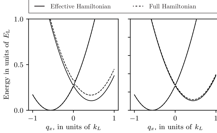
Figure 6: Solid lines: Dispersion relation from RWA Hamiltonian (Equation 8.8) as a function of q_x for \Omega_{i,j} = 1.5 E_L and \delta_i = 0 . Dashed lines: Dispersion relation computed for the full Floquet Hamiltonian. We considered \omega_{zx} = 2\omega_{xy} and \omega_{zy} = 3\omega_{xy} in both cases so the separation between Floquet manifolds is \omega_{xy} . In the left panel \omega_{xy} = 83.24 \text{ kHz} as in our experiments and in the right panel \omega_{xy} = 416.2 \text{ kHz} . As the spacing between Floquet manifolds becomes we get a better agreement between the spectra of the RWA and Floquet Hamiltonians.
