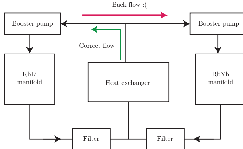
Figure 3: Simplified schematic of the shared water cooling manifold.
