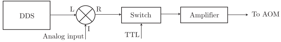
Figure 8: Setup used to drive the AOMs controlling the power and frequency of Raman beams. A similar setup is used to drive a coil used to generate high-power RF fields at the atoms.
