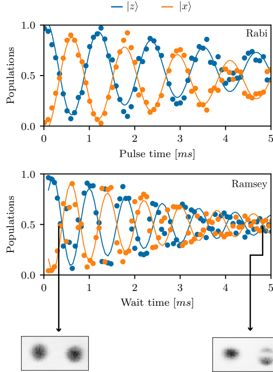
Figure 9: Loss of contrast in coherent oscillations. A Rabi oscillation (top) between the |z\rangle and |x\rangle states with \Omega_p/2\pi = 870 Hz decays by 1/e in 4.6 ms and a Ramsey oscillation (middle) with about 1 kHz frequency decays in about 3 ms. The gradients in \Omega lead to phase separation of dressed states and loss of contrast for longer pulse/wait times.
