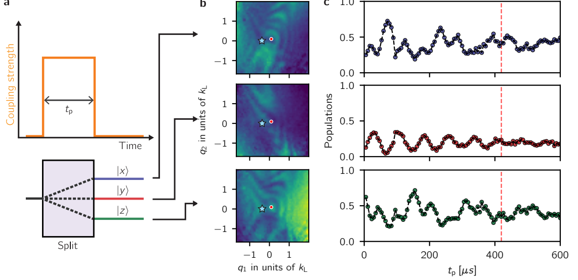
Figure 10: a Fourier spectroscopy protocol. We applied the Raman lasers for a variable time t_p : a Rabi-type atomic interferometer analogous to a three-port beam splitter. b Probabilities as a function of quasimomentum for a fixed Raman pulse time t_p = 420 \mu\text{s} c Dynamics of the final populations of the |xyz\rangle states with quasimomentum (q_1, q_2) = (-0.55, -0.18) k_L (blue star in panels b ) after initializing the system in the |z\rangle state.
