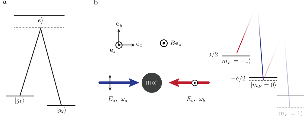
Figure 3: a. A Raman transition is a two photon process that couples two ground states through and intermediate far detuned state. b. We induce Raman transitions using a pair of cross-polarized laser beams and we set the difference in their angular frequencies close to the Zeeman splitting between two consecutive |m_F\rangle states.
