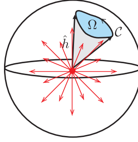
Figure 4: For a two-level system, the Berry curvature from a Dirac point can be viewed as a Dirac monopole in momentum (parameter) space. The Chern number can be interpreted as the flux from the monopole on the solid angle subtended by the vector \hat{h}(\mathbf{k}) or alternatively as the number of times \hat{h}(\mathbf{k}) wraps around a unit sphere.
