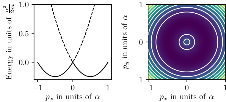
Figure 1: The Rashba dispersion relation has a Dirac point located at \mathbf{k} = 0 and a degenerate ground state that is described by the ring k_x^2 + k_y^2 = \alpha^2 .
