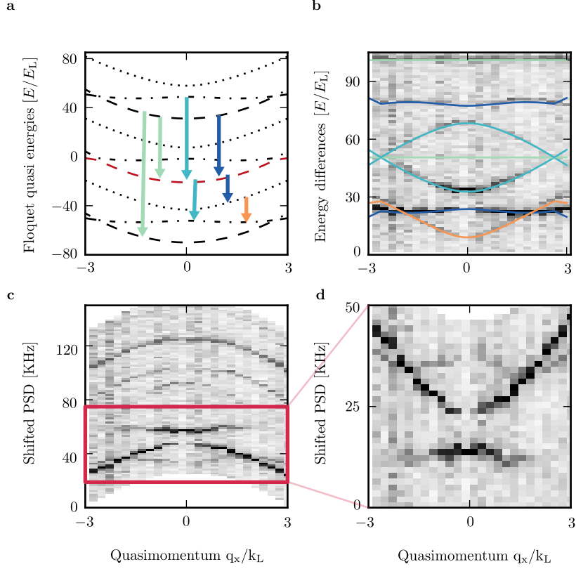
Figure 7: a Floquet quasi-energy spectrum of a SOC Hamiltonian with periodic coupling strength. The red line represents the eigenstate that has the largest overlap with the initial |m_F = 0\rangle state. The arrows indicate the energies of the states that have non-zero overlap with the initial state and can be measured with Fourier transform spectroscopy. b PSD of the occupation probability and numerically calculated energy differences between the levels indicated by the arrows on panel a. c PSD shifted by a quadratic term -\hbar^2 q_x^2 / 2m^* . The red box indicates the region of interest where we can recover the SOC spectrum. d We invert the frequency axis and shift it by \delta\omega .
