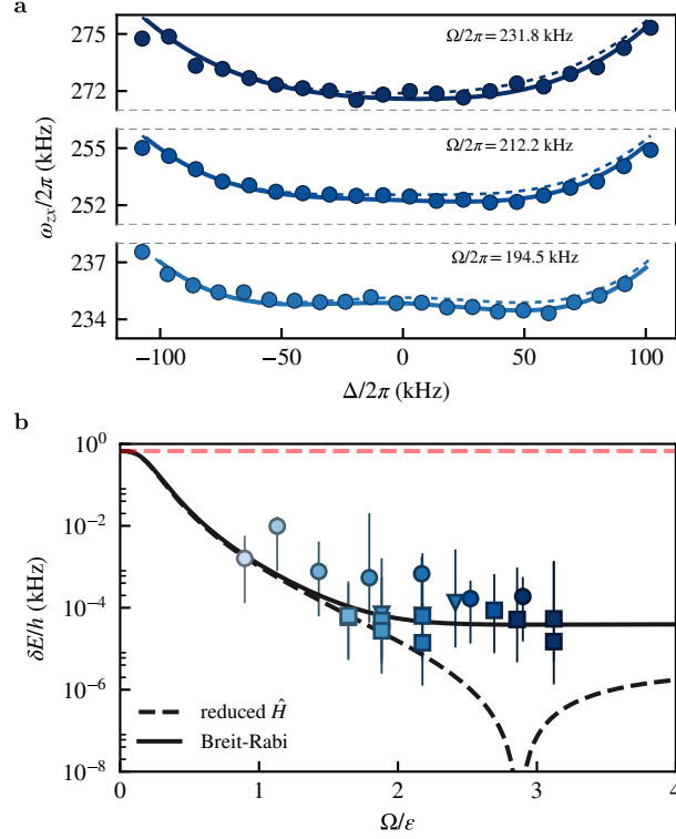
Figure 6: a. Transition frequency \omega_{zx}/2\pi for three values of \Omega/2\pi . The dashed curves correspond to Equation 6.7, while the solid curves use the Breit-Rabi expression. b. The change in energy from our experimental detuning fluctuations as measured in the |m_F\rangle basis is \delta\Delta/2\pi = 0.67 kHz (red dashed line). Triangles correspond to |xyz\rangle spectroscopy data, squares to side-of-peak \pi -pulse data, and circles to double-dressed data. The black dashed (solid) curve was calculated using Equation 6.7 (the Breit-Rabi expression). The shading of the data points corresponds to the Rabi frequencies in Figure 8.
