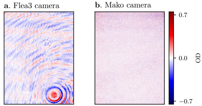
Figure 12: OD computed using two consecutive probe images without atoms. a. With the Flea3 camera images are spaced by \sim 30 ms. Changes in the probe result in fingers in the OD. b. With the Mako camera images are spaced by \sim 150 \mu\text{s} .
