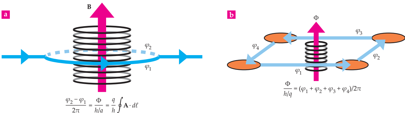
FIGURE 3. PHASE ENGINEERING. Quantum mechanical particles experience magnetic fields by acquiring Aharonov–Bohm (AB) phases. (a) In an AB interferometer, a magnetic field \mathbf{B} is confined to the interior of a solenoid and is zero outside it. Nevertheless, a particle that travels on opposite sides of the solenoid will acquire a phase difference proportional to the enclosed magnetic flux \Phi . That flux equals the line integral of the vector potential \mathbf{A} around the solenoid. The charge is specified by q . (b) Particles that tunnel in a lattice experience an applied magnetic field in much the same way as in the AB effect. Their tunneling motion from one site to another acquires a so-called Peierls phase, such that the sum of the phases around a closed loop equals the enclosed flux.
